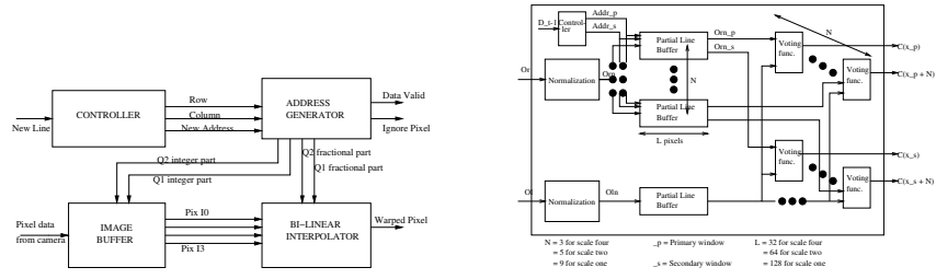
Fig. 3. Architecture of Image Rectification Unit. Fig. 4. Modified correlation unit with two shiftable windows.
