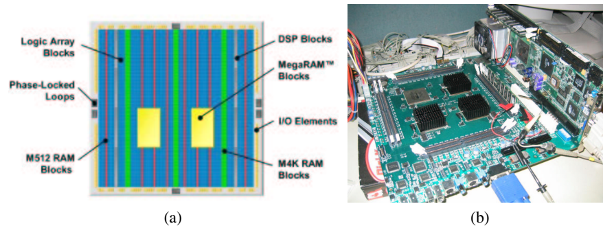
Fig. 1. (a) Typical features of a modern FPGA [3]. (b) Transmogrieffier-4 reconfigurable computing board [7]
