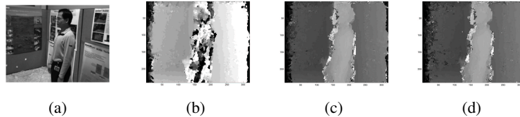
Fig. 8. In sequence MDR-2, we see that the proposed range-expansion algorithm (c) performs significantly better than the original algorithm (b). The disparity map using a larger primary correlation window of 13 pixels (d) is a slight improvement over (c).
